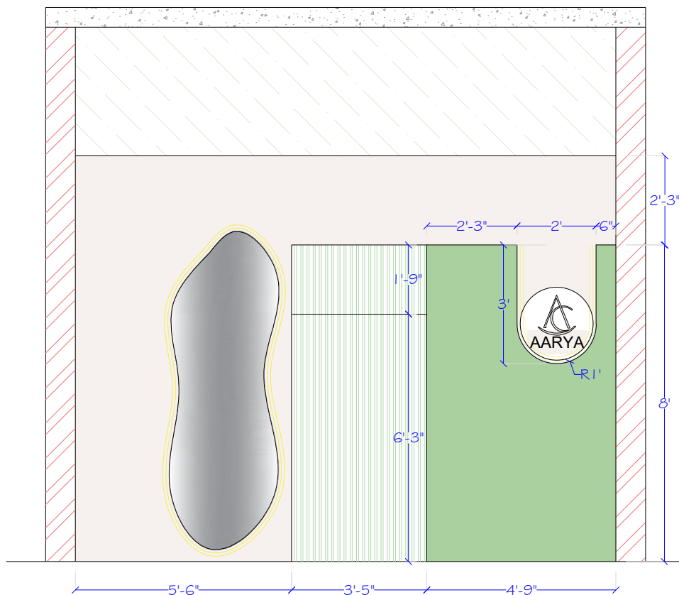
WALL ELEVATION D MEASUREMENT
