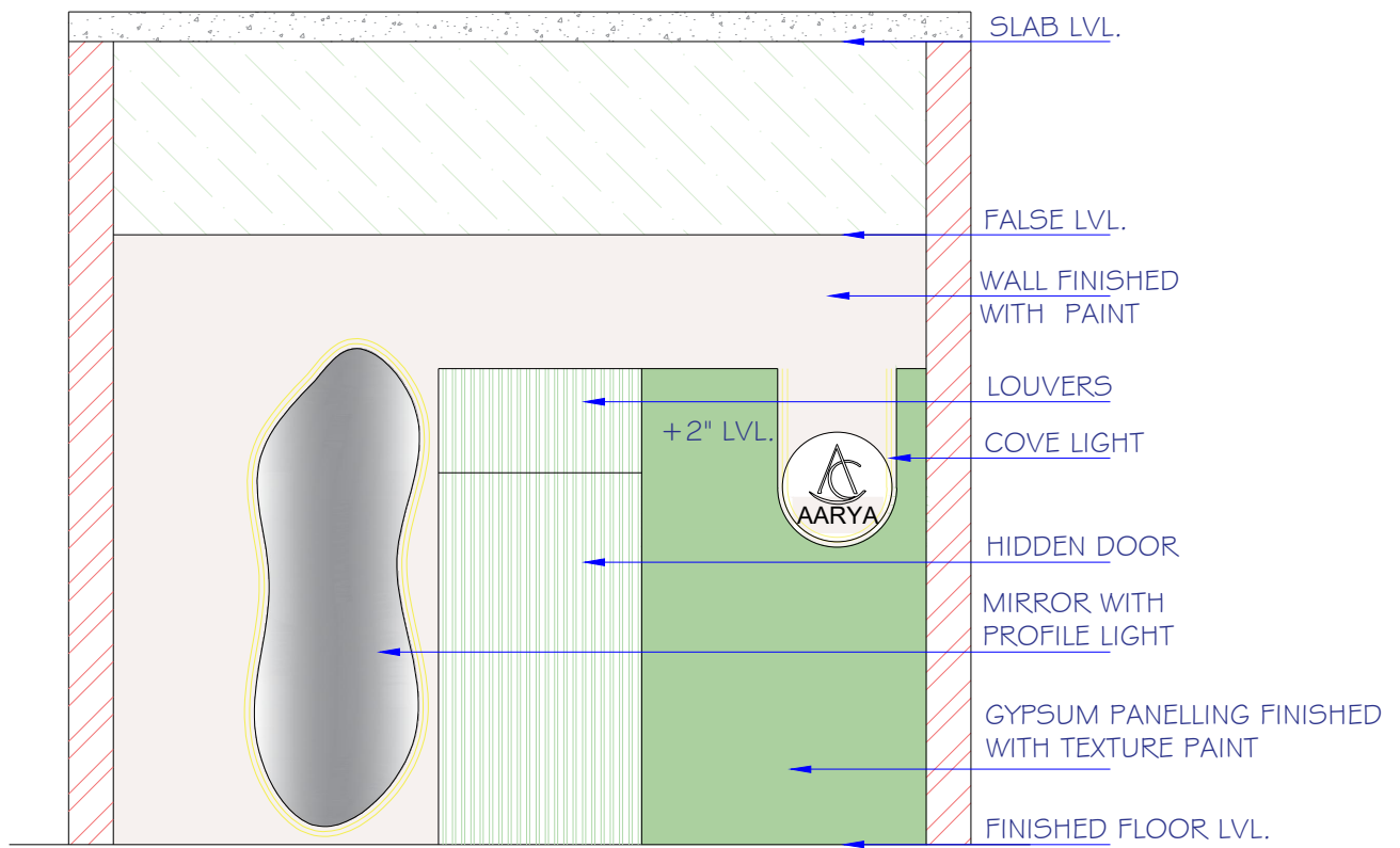
WALL ELEVATION D DETAIL
